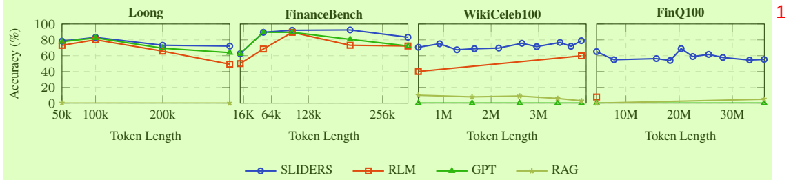
Figure 5: Accuracy vs. token length across benchmarks. 2
