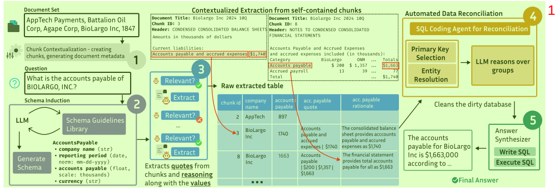
Figure 3: SLIDERS overview showing the process of (1) Contextualization of chunks, (2) Inducing the schema, (3) Structured Extraction, (4) Data Reconciliation, and (5) Question Answering over the final database. An example from the Loong benchmark.
